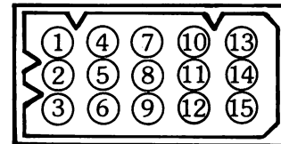
Keyboard Connector Viewed from end of cable plug
