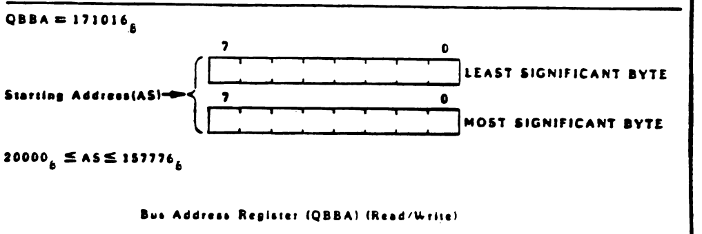
Figure E-3 QBDC . QBTC . QBBA Registers 0074-001
