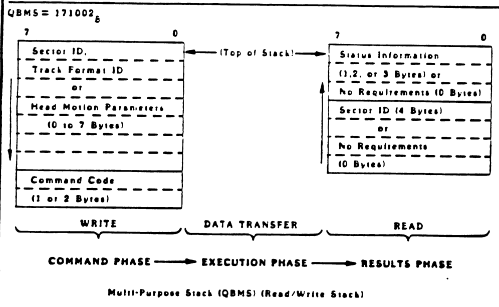
Figure E-2 QBCS , QBMS Registers
